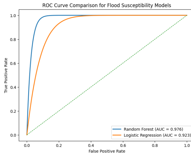
Figure 5. AUC Scores for Models
