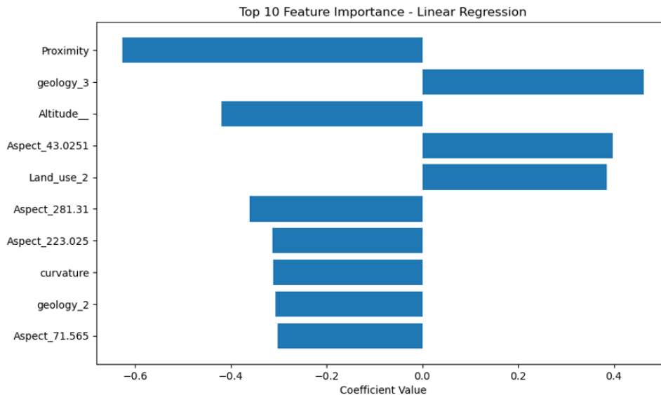
Figure 7. Logistic Regression (Mean Squared Error: 2.778, R^2 Score: 0.444)
