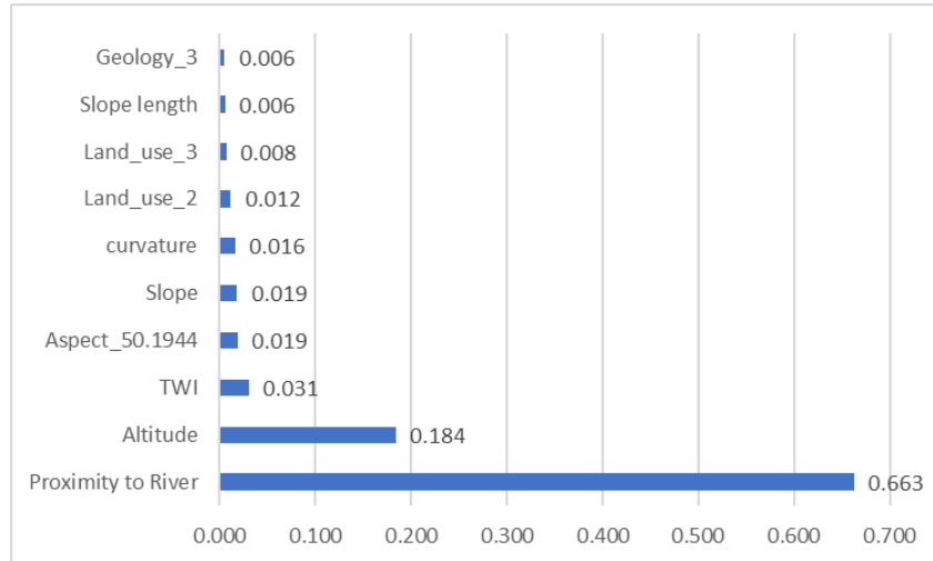
Figure 6. RF Feature Importance (Mean Squared Error: 0.633, R^2 Score: 0.76175)
