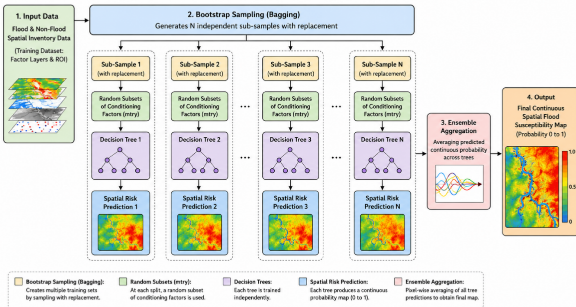
Figure 3. Random Forest Algorithm Structure (Author's Analysis, 2026)
