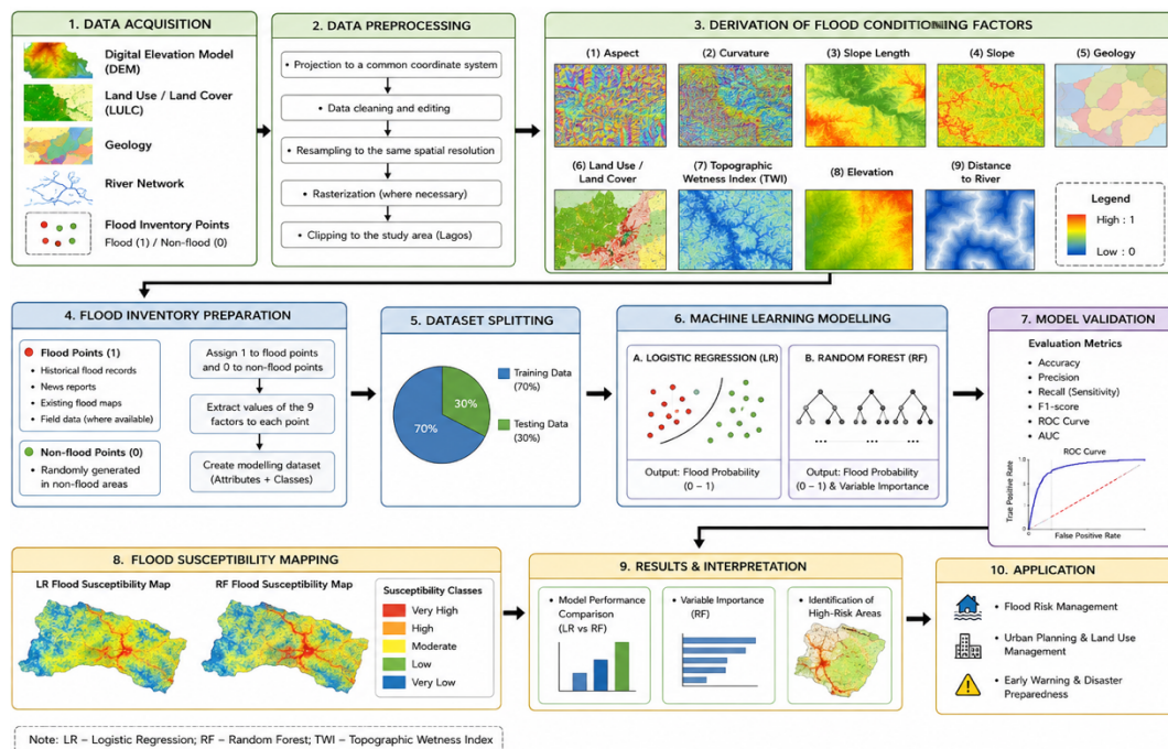
Figure 4. Methodology Workflow
